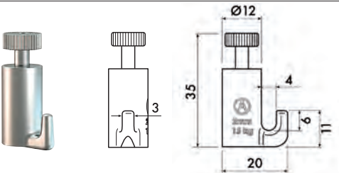
9.4261 15 kg
