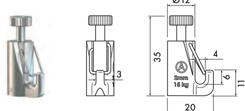
9.4264 15 kg
